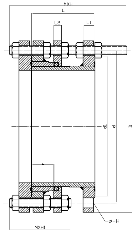
Dimensions(mm)
